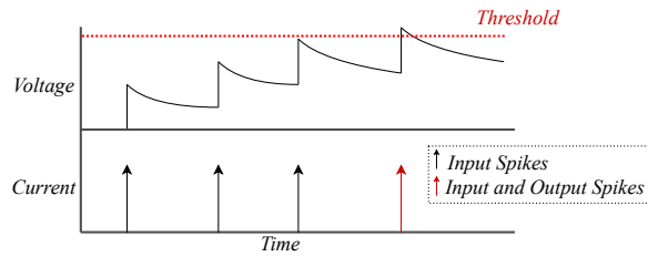
Fig. 1. Illustration of a LIF model. Change of voltage caused by the input spikes. An output spike is observed when the voltage reaches a threshold.
