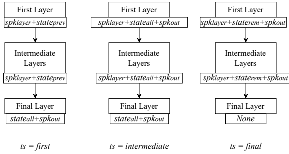
Fig. 3. Checkpointing strategy based on timestep and model layer.
